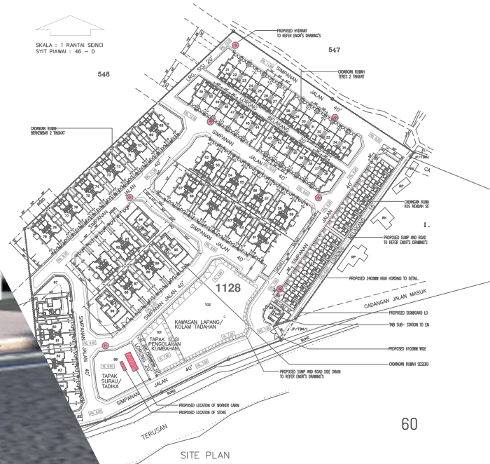
SITE PLAN
